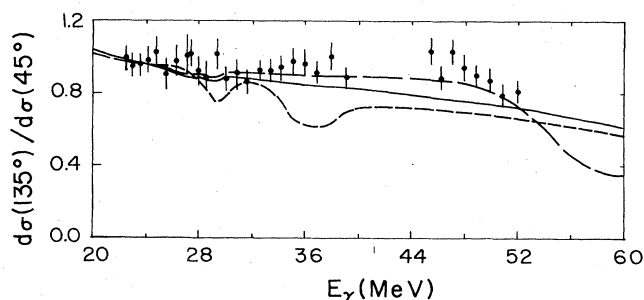
FIG. 7. Ratio of scattering cross sections, d\sigma(135^{\circ})/d\sigma(45^{\circ}) , for carbon. The solid curve is calculated from \sigma_{\gamma}^{E1} inferred from the angle-averaged scattering data. The long dashed curve is calculated from this \sigma_{\gamma}^{E1} plus \sigma_{\gamma}^{E2} in the form of a Lorentzian of width 12 MeV, centered at 55 MeV, and exhausting 1 TEWS. The short dashed curve is calculated by assuming \sigma_{\gamma}^{E2} = \sigma_{\gamma}^{\text{expt}} - \sigma_{\gamma}^{E1} .
