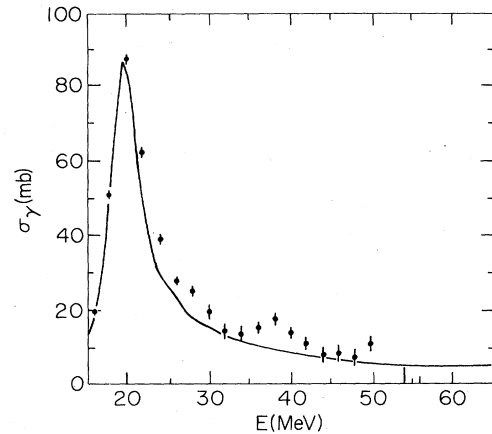
FIG. 9. Photoabsorption cross section for calcium. The points are the previously reported values for \sigma_\gamma^{\text{expt}} and the curve is the \sigma_\gamma^{E1} inferred from the angle-averaged scattering data.
